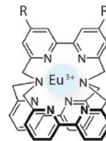
FIGURE: \text{Eu}^{3+} Trisbipyridine Structure.
