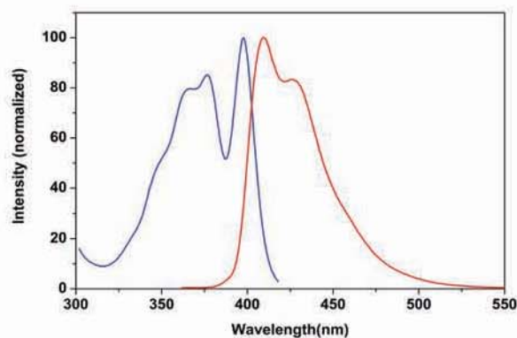
Figure 3.2 The excitation and emission spectra of iFluor™ 405 Goat Anti-Rabbit IgG conjugate (Cat# 16604) in PBS buffer (pH 7.2).
