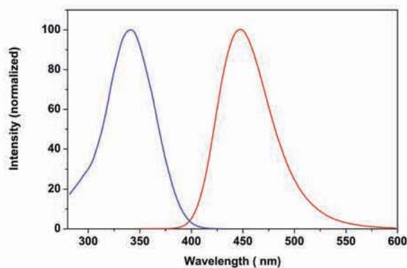
Figure 3.1 The excitation and emission spectra of iFluor™ 350 Goat Anti-Rabbit IgG conjugate (Cat# 16600) in PBS buffer (pH 7.2).
