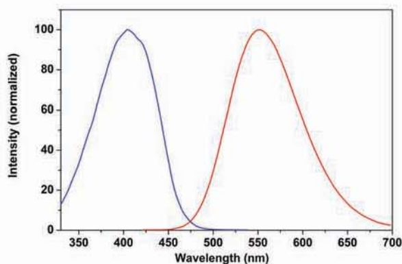
Figure 4.3 The excitation and emission spectra of mFluor™ Violet 540 Goat Anti-Rabbit IgG conjugate in PBS buffer (pH 7.2).
