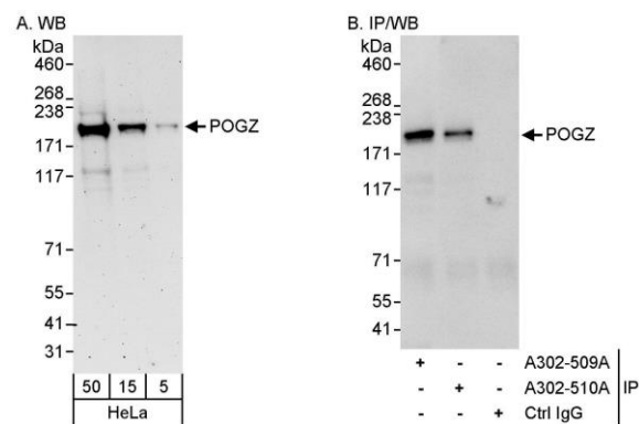
Detection of human POGZ by western blot and immunoprecipitation. Samples: Whole cell lysate (5, 15 and 50 µg for WB; 1 mg for IP, 20% of IP loaded) from HeLa cells. Antibodies: Affinity purified rabbit anti-POGZ antibody A302-509A used for WB at 0.1 µg/ml (A) and 1 µg/ml (B) and used for IP at 3 µg/mg lysate. POGZ was also immunoprecipitated by rabbit anti-POGZ antibody A302-510A, which recognizes a downstream epitope. Detection: Chemiluminescence with exposure times of 3 minutes (A) and 10 seconds (B).
