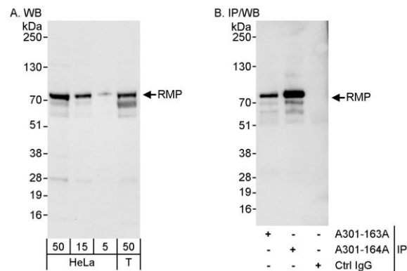
Detection of human RMP by western blot and immunoprecipitation. Samples: Whole cell lysate from HeLa (5, 15 and 50 \mu g for WB; 1 mg for IP, 20% of IP loaded) and HEK293T (T; 50 \mu g) cells. Antibodies: Affinity purified rabbit anti-RMP antibody A301-163A used for WB at 0.04 \mu g/ml (A) and 1 \mu g/ml (B) and used for IP at 3 \mu g/mg lysate. RMP was also immunoprecipitated by rabbit anti-RMP antibody A301-164A, which recognizes a downstream epitope. Detection: Chemiluminescence with exposure times of 30 seconds (A) and 10 seconds (B).
